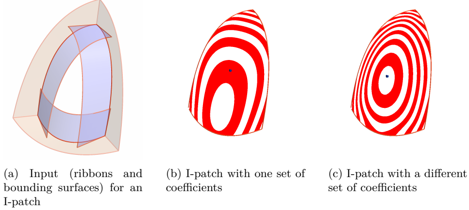
Figure 1: I-patches. Figure from [14]
