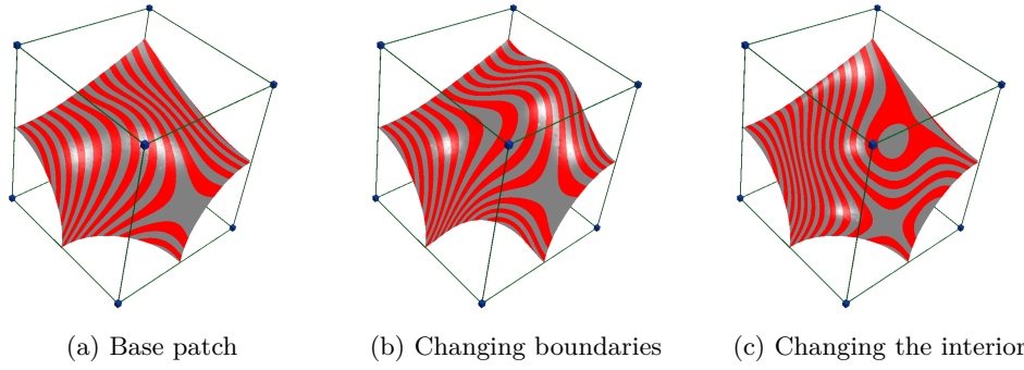
Figure 4: Corner I-patches with the same corner interpolants and different coefficients
