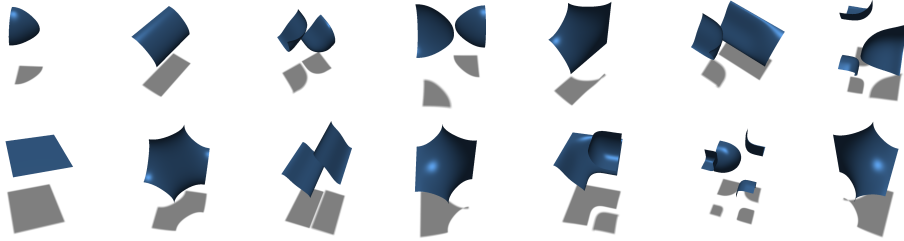
Figure 5: The 14 non-empty basic configurations of Marching Cubes represented with corner I-patches (in the same order as in [12])
